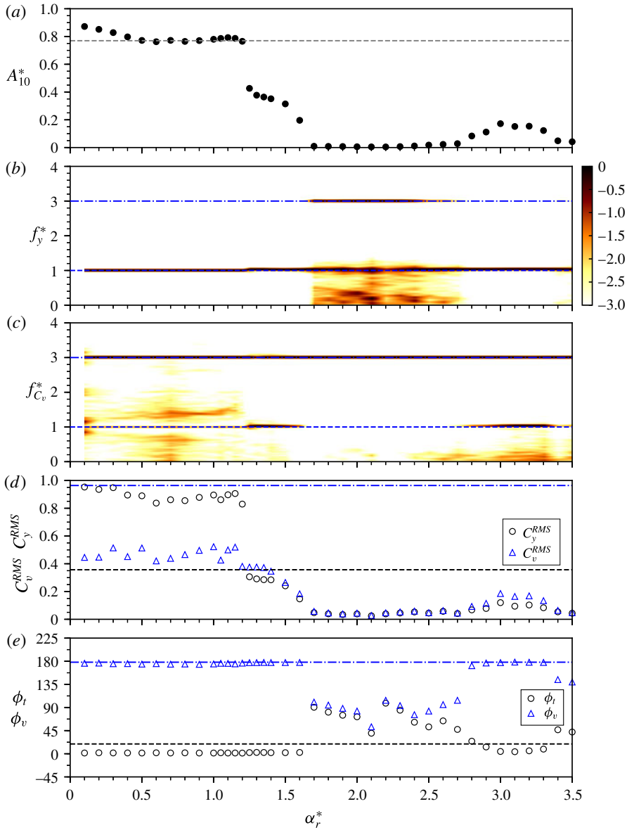
FIGURE 11. (Colour online) Vibration response quantities as a function of the forcing velocity ratio ( \alpha_r^* ) at a fixed forcing frequency ratio of f_r^* = 3.0 and at U^* = 5.5 . For further details on the symbols and lines in the plots, refer to the caption of figure 5.
