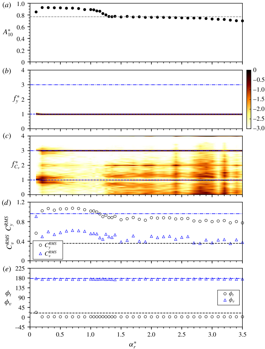
FIGURE 10. (Colour online) Vibration response quantities as a function of the forcing velocity ratio ( \alpha_r^* ) at a fixed forcing frequency ratio of f_r^* = 1.0 and at U^* = 5.5 . For further details on the symbols and lines in the plots, refer to the caption of figure 5.
