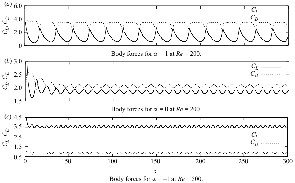
FIGURE 18. Time histories of the unsteady lift and drag coefficients at representative values of the rotation rate.
