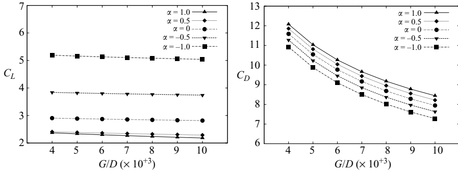
FIGURE 3. Variation in the lift and drag forces with varying gap ratio at Re = 20 .
