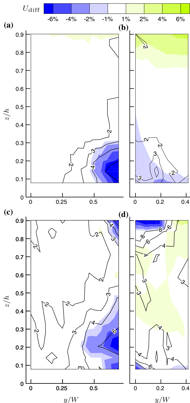
Fig. 5 Comparison of flow uniformity in the empty test section (left side) with the flow in the sub-channel at model location (right side) at two freestream velocities: a, b U_\infty = 0.045 m/s, c, d U_\infty = 0.135 m/s. The colour contours show U_{diff} ; the contour lines represent Tu[\%] . ( \alpha = 0.154 , g = 5 mm)
