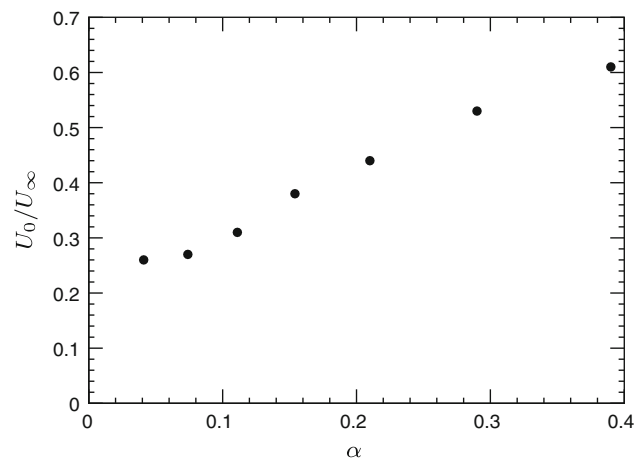
Fig. 3 Freestream velocity reduction inside the sub-channel as a function of screen porosity \alpha , measured at model location ( x = L/3, y = 0, z = h/2 ) and U_\infty = 0.09 m/s. Error bars are smaller than the symbols
