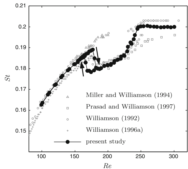
Fig. 9 Measurement of shedding frequency of a circular cylinder in the sub-channel (filled circles), in comparison to the literature data. The arrows mark the path through the hysteretic discontinuity when increasing (arrow down) and when decreasing (arrow up) the Reynolds number
