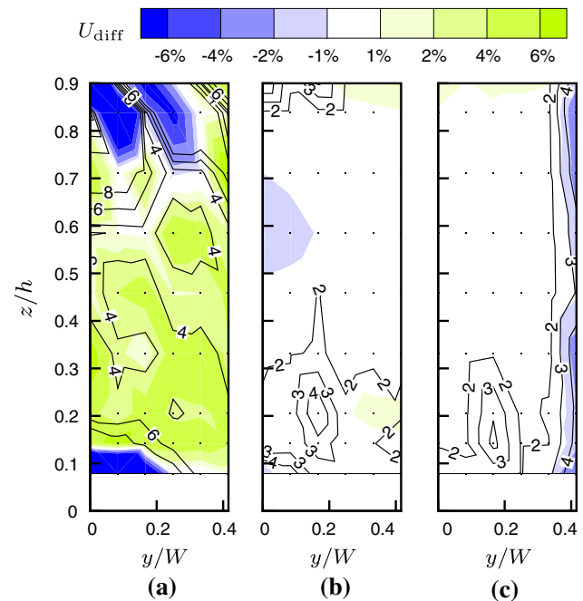
Fig. 8 Flow uniformity at model location for three different screen porosities \alpha : a 0.041, b 0.154, c 0.39. The colour contours show U_{\text{diff}} ; the contour lines represent Tu [%]. The dots mark LDV sampling points. ( U_\infty = 0.090 m/s, g = 5 mm)
