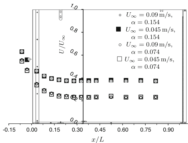
Fig. 4 Development of streamwise velocity inside the sub-channel along the centreline. Data for two pump speeds and two values of \alpha are overlaid on a side view of the sub-channel. Error bars are smaller than the symbols. The flow is from left to right
