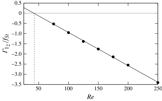
FIGURE 7. Coefficient \Gamma_{12}/f_{st} as a function of Re , f_d/f_{st} = 1 . The solid black line is a linear fit, \Gamma_{12}/f_{st} = -0.0163Re + 0.683 , to the data points. The match between the measurements and the fit is excellent. Extrapolation of the fit shows that \Gamma_{12} = 0 at Re \simeq 42 , indicating that the frequency will cease to decrease with increasing A^* at this value. This value of Re is just below that where vortex shedding from a stationary cylinder begins ( Re \simeq 47 ).
