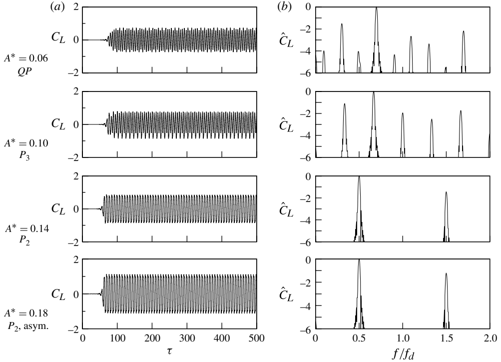
FIGURE 6. (a) Time histories of the lift coefficient C_L and (b) portions of the frequency spectra obtained from taking the Fourier transform of the lift coefficient history; Re = 175 , f_d/f_{St} = 1.4 . The amplitude of oscillation increases from top to bottom. The change in signature of the time history and spectrum as the flow moves from quasi-periodic to the various synchronized modes is clear. The data presented are the same as those of figure 5.
