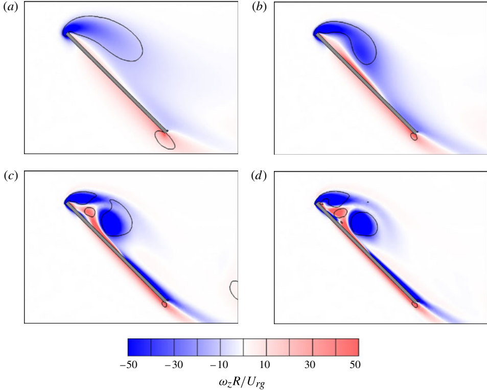
FIGURE 4. (Colour online) Contours of spanwise vorticity ( \omega_z R/U_{rg} ) at 50% span for Reynolds numbers of (a) 120, (b) 300, (c) 750 and (d) 1500. Solid lines are contours of constant Q criterion. Images show the instantaneous flow structures at 270^\circ of rotation.
