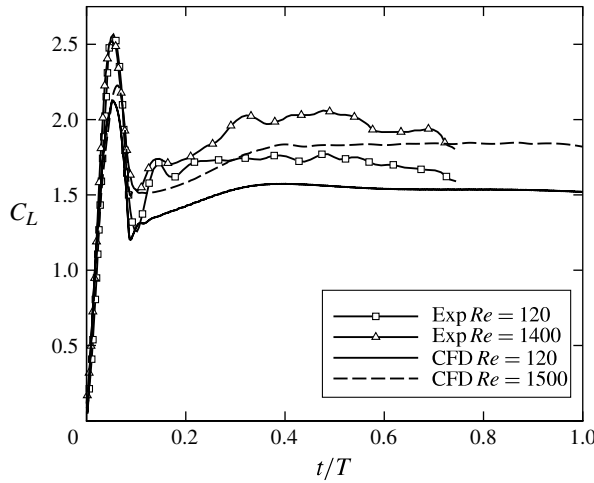
FIGURE 7. Lift coefficient time history for an AR = 2.91 wing compared with the experimental results of Birch et al. (2004).
