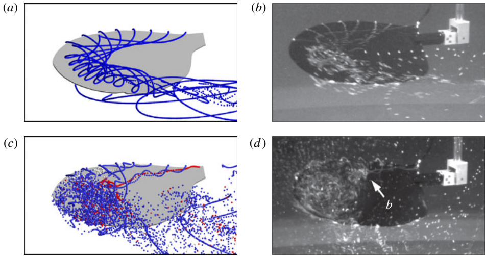
FIGURE 2. (Colour online) Comparison of numerical particle tracking flow visualization results at (a) Re = 120 and (c) Re = 1500 with air bubble flow visualizations of Lentink & Dickinson (2009b) (reproduced with permission) at (b) Re = 110 and (d) Re = 1400 .
