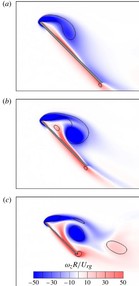
FIGURE 11. (Colour online) Contours of time-averaged spanwise vorticity ( \omega_z R/U_{rg} ) at 50% span for wings at Re = 300 : (a) AR = 2.91 ; (b) AR = 5.1 ; and (c) AR = 7.28 . Solid lines are contours of constant Q criterion. Flow field has been averaged over the quasi-steady period ( 0.36 \leq t/T \leq 1.0 ).
