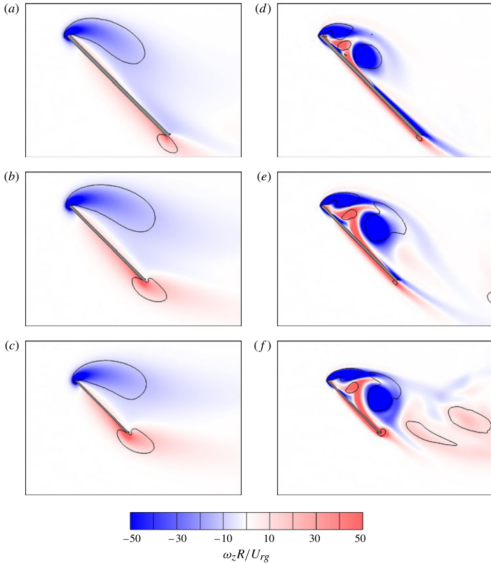
FIGURE 13. (Colour online) Contours of time averaged spanwise vorticity ( \omega_z R/U_{rg} ) at 50% span for different AR wings at span-based Reynolds numbers of (a–c) Re_R = 613 and (d–f) Re_R = 7667 : (a,d) AR = 2.91 ; (b,e) AR = 5.1 ; (c,f) AR = 7.28 . Solid lines are contours of constant Q criterion. The flow field has been averaged over the quasi-steady period ( 0.36 \leq t/T \leq 1.0 ).
