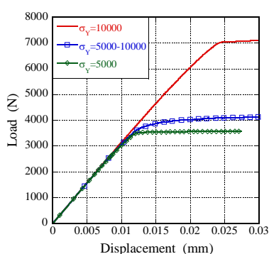
Fig 11 Load displacement relationship for plastic deformation dominant failure.
