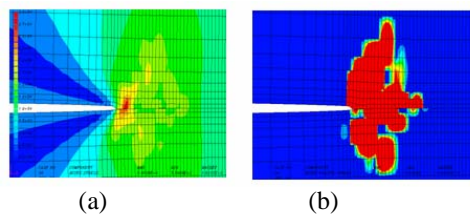
Fig. 10 Distribution of Mises stress and Plastic strain.
