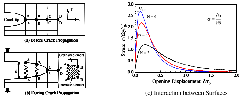
Fig 1 Outline of the “Interface Element”.
