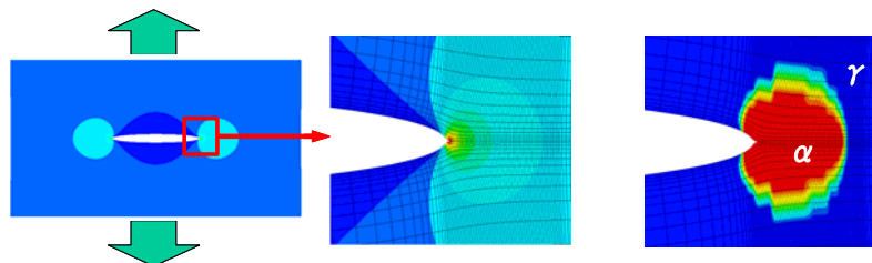
Fig 2 Model, applied load, deformed shape, mean stress at crack tip and austenite \gamma (Blue) – martensite \alpha (Red) distribution for \sigma_{cr} = 3000 \text{ MPa} and \alpha = 0 .
