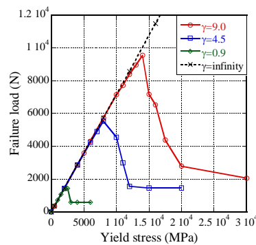
Fig.8 The influence of surface energy \gamma on failure strength.
