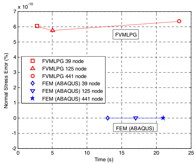
Figure 20: Computational efficiency of the FVMLPG and the FEM in the normal stress
